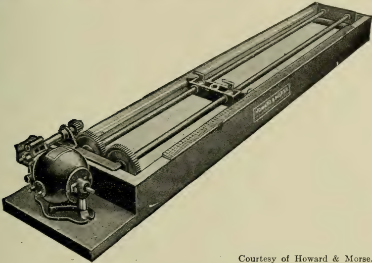
FIG. 167.—Smith Ductility Machine.
